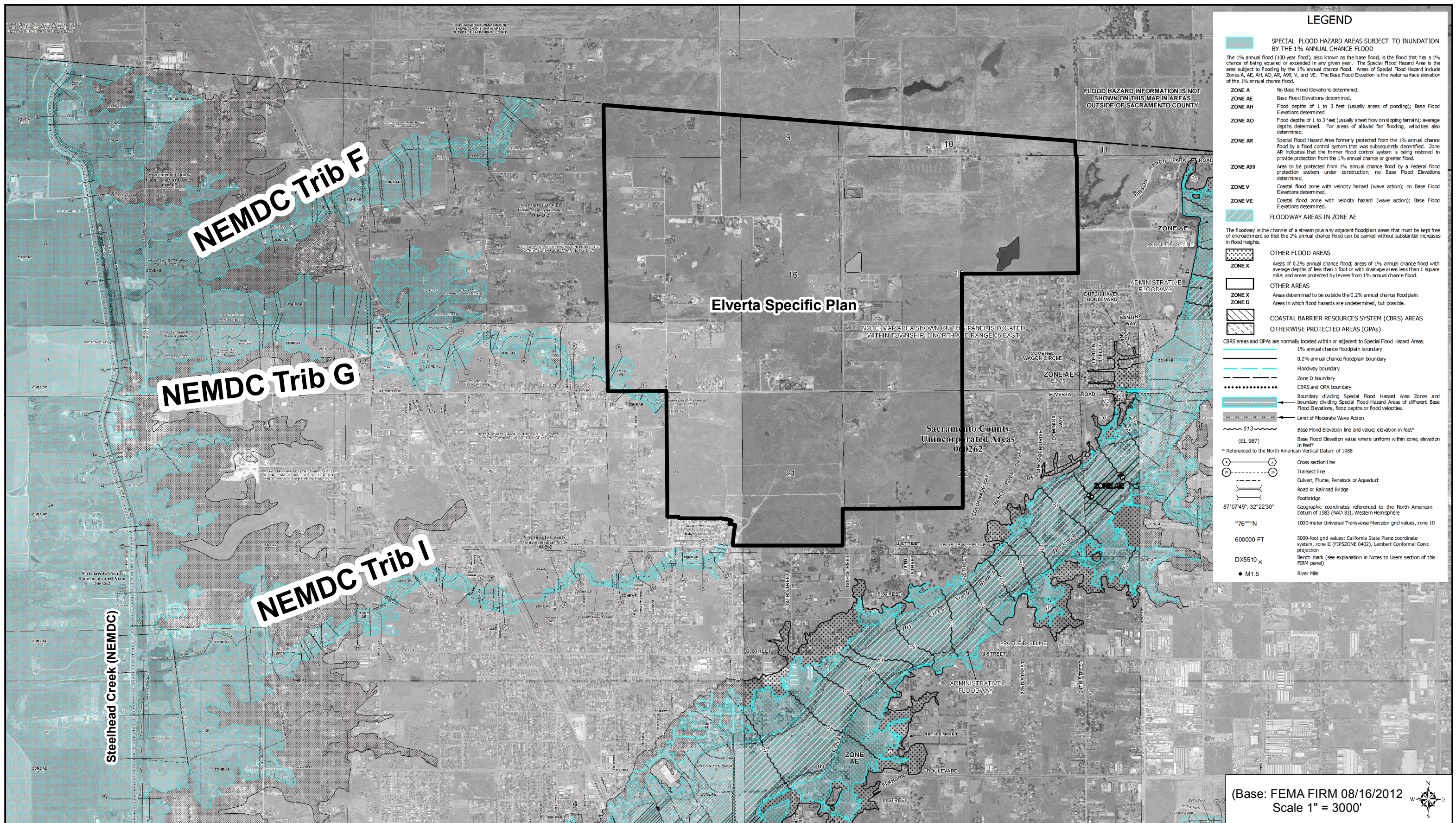
Exhibit 7 : FEMA Regional Floodplain Delineation (Datum : NGVD88)
