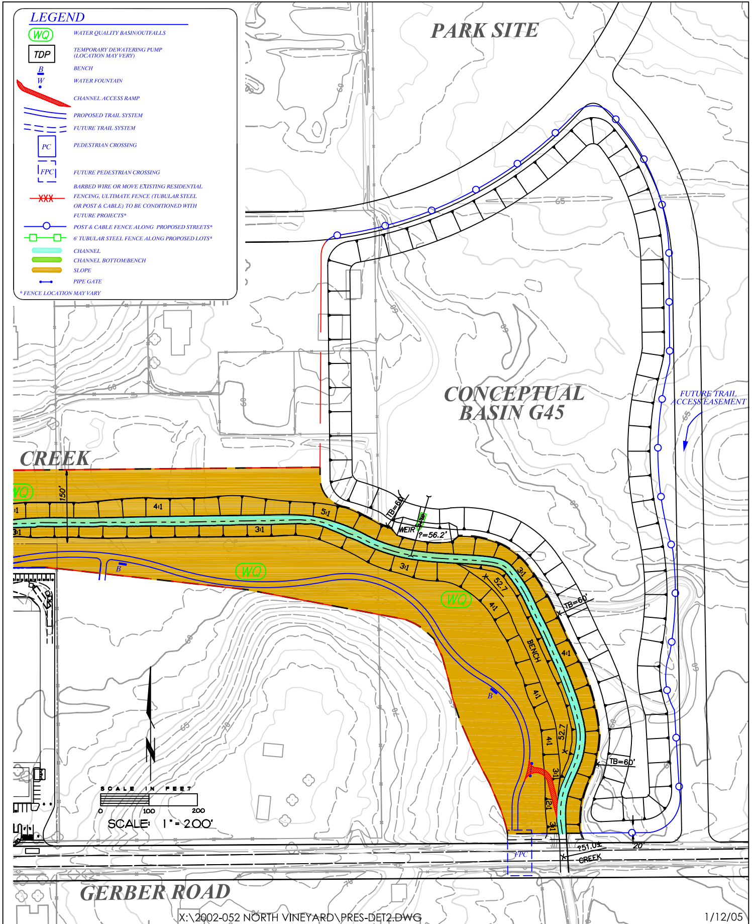
FIGURE 15. Preserve Detail Sheet-Sheet 12
