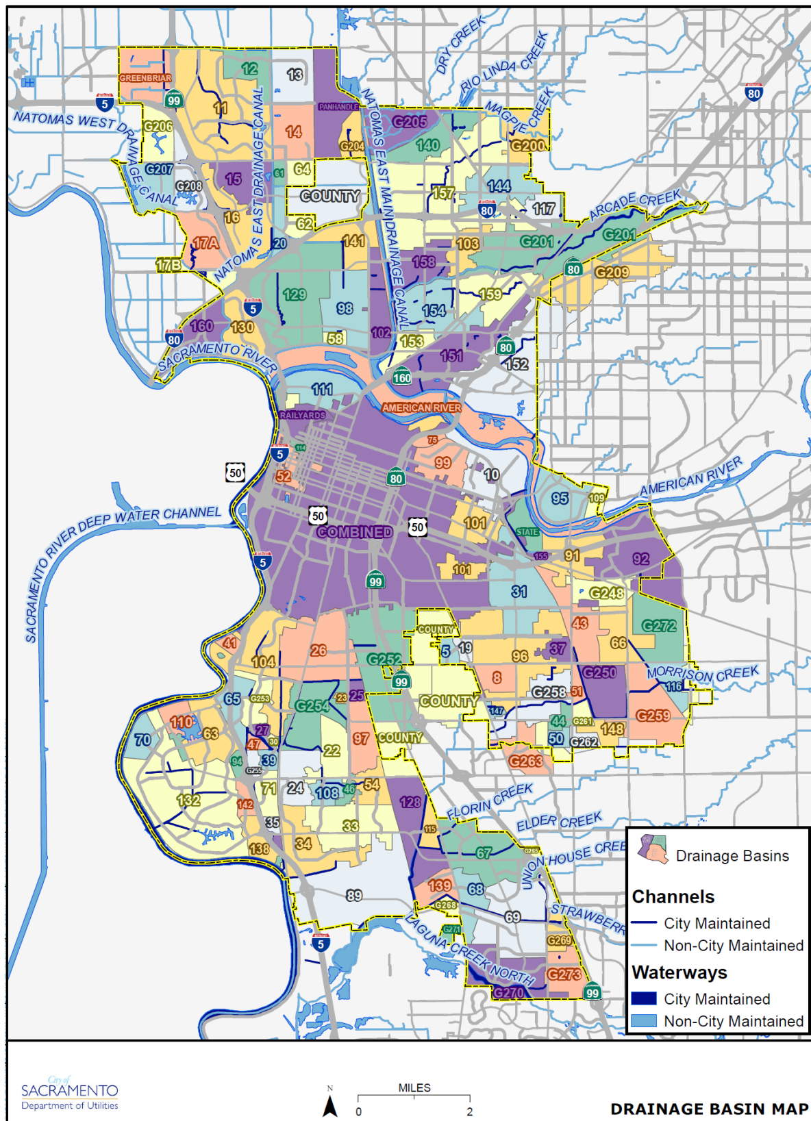
Figure F-48 City of Sacramento – Drainage Basins
